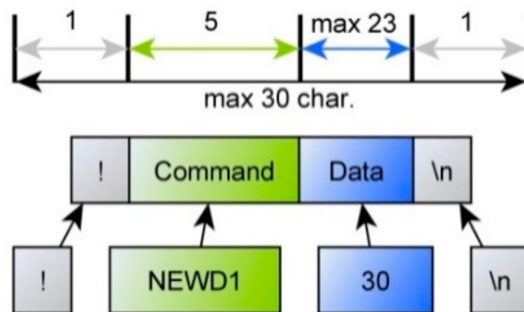
Figure 11. Structure of a data package.
