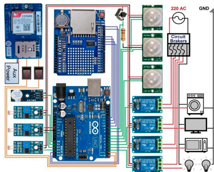
Figure 12. Wiring diagram of the system's components.
