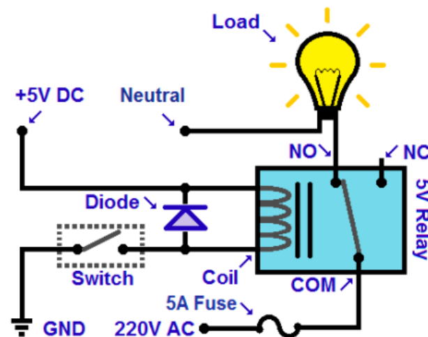
Figure 4. Diagram of the relay modules used to control different loads in the home.
