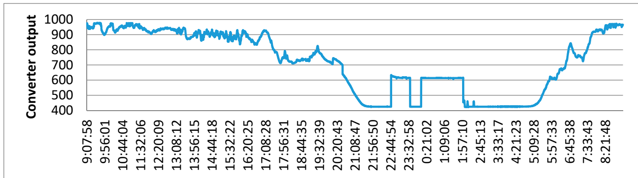
Figure 3. Indoor light intensity fluctuation in 24 h.
