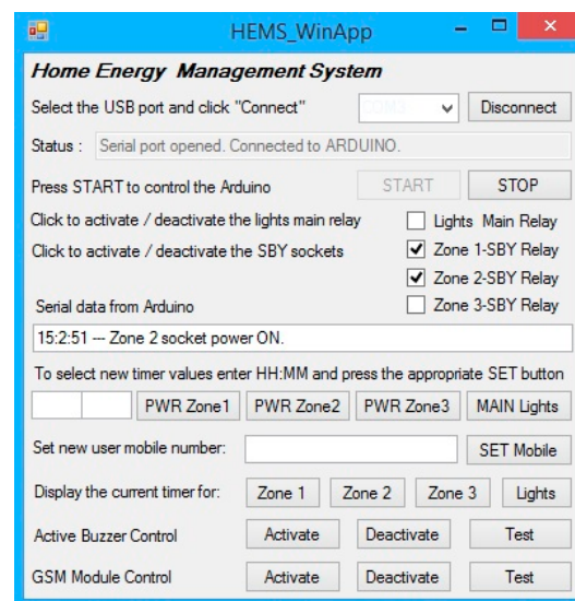
Figure 10. Windows-based Visual C# App.
