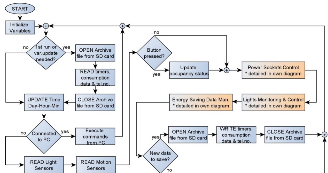
Figure 6. Flow diagram of the system's data management and back-up functions.
