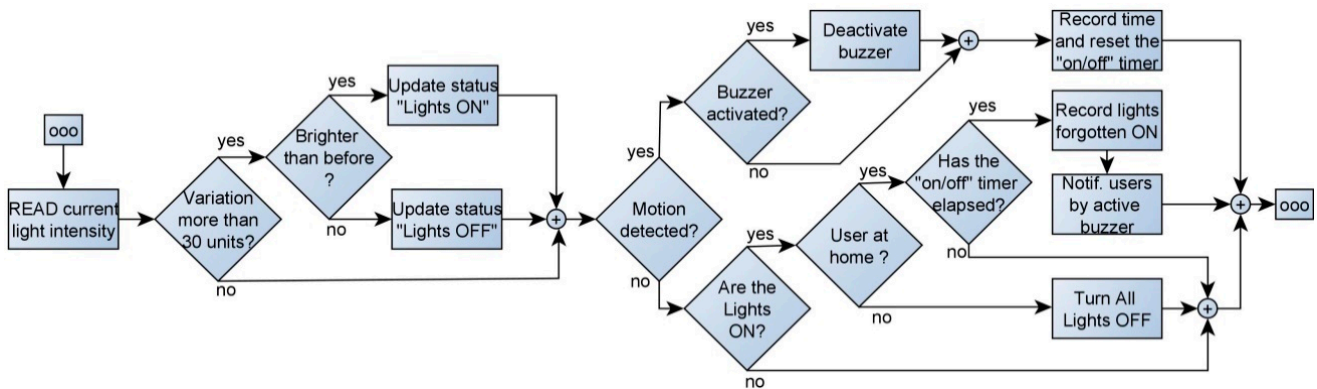
Figure 7. Flow diagram of the system’s lights monitor and control function.
