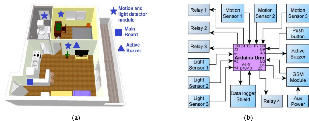
Figure 1. Home energy management system. (a) The placement of system components in typical homes. (b) Home energy management system's architecture.
