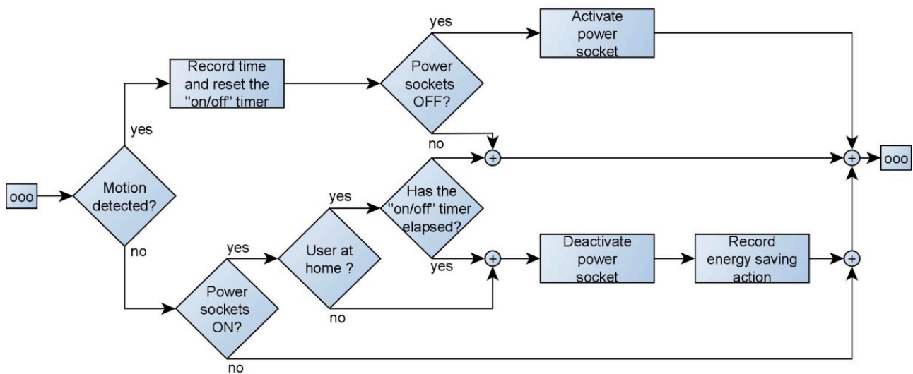
Figure 8. Flow diagram of the power sockets control function.
