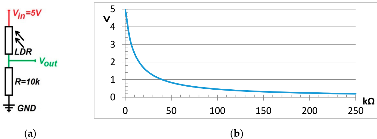
Figure 2. Converting brightness fluctuations in voltage variations. (a) The voltage divider's diagram; (b) voltage variation as a function of resistance.
